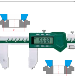
Digital Rtj Ring Groove Calipers
