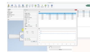
CG analysis
