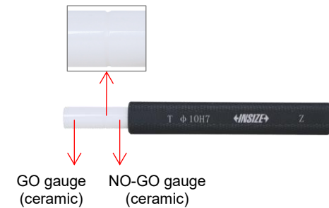
Ceramic Plain Plug Gauges (Single End) 6333
